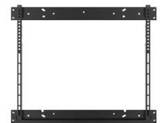
Universal VESA Bracket
